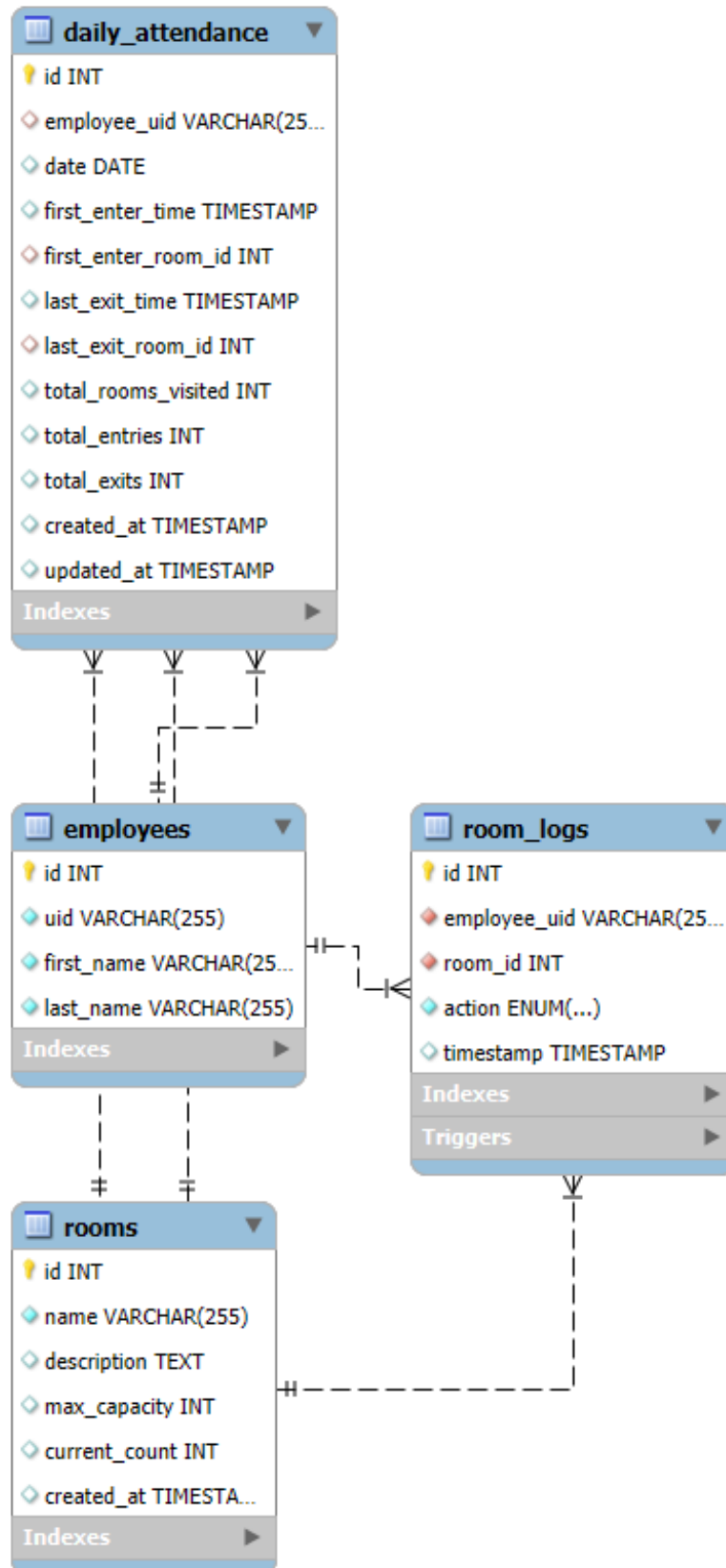
Gambar 1.1 ERR Diagram Database MySQL
